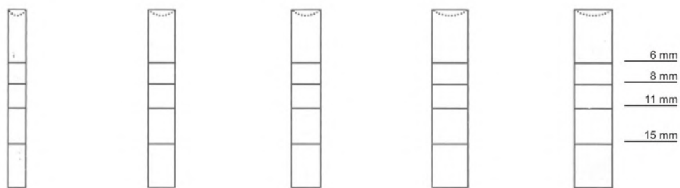
Ø 2 mm 1BCC Ø 3 mm 2BCC Ø 3.3 mm 3BCC Ø 4 mm 4BCC Ø 5 mm 5BCC
